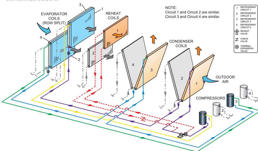
REFRIGERANT SCHEMATIC
