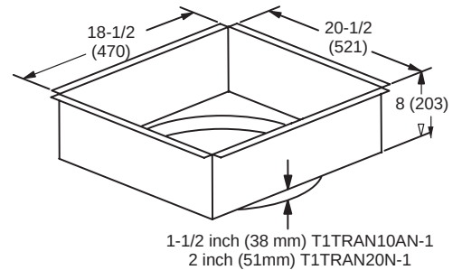
SUPPLY TRANSITION
