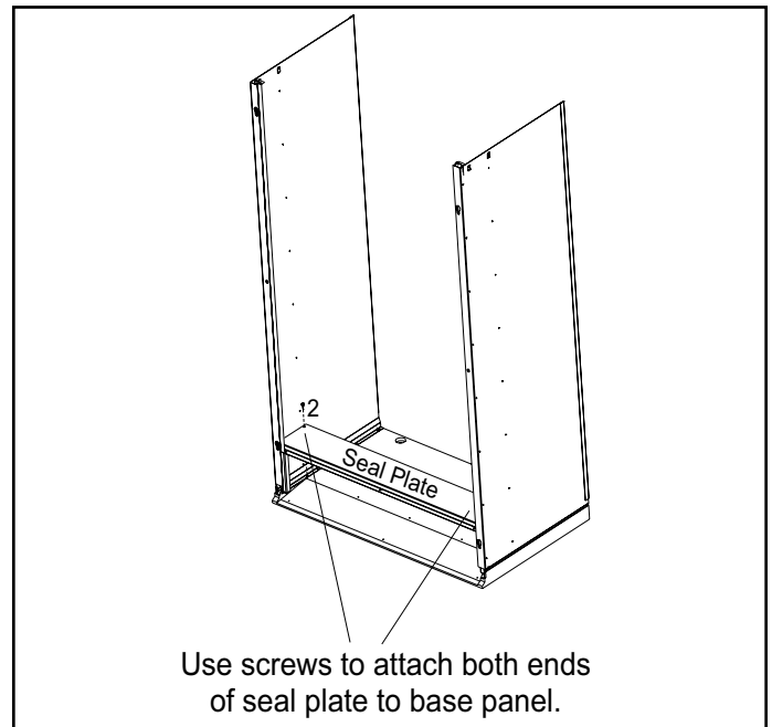
Figure 3. Installing Bottom Seal Plate (ASLEEVE2 kits only)
