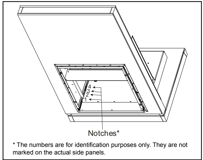
Figure 13. Identifying Side Panel Notches
