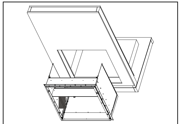
Figure 8. Installing Wall Sleeve from Outside
