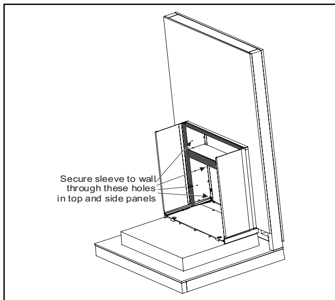
Figure 10. Securing Wall Sleeve to Wall Opening (if mounting angles were not installed)
