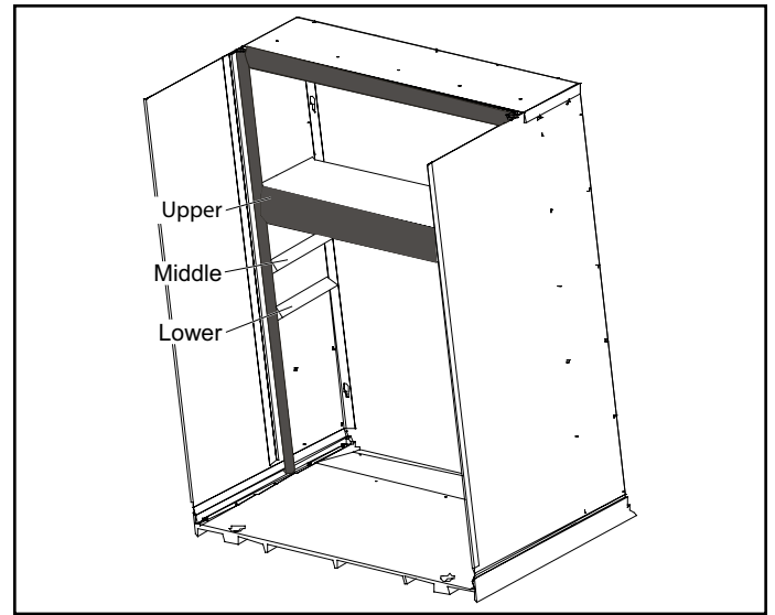
Figure 5. Installing Divider Panel
