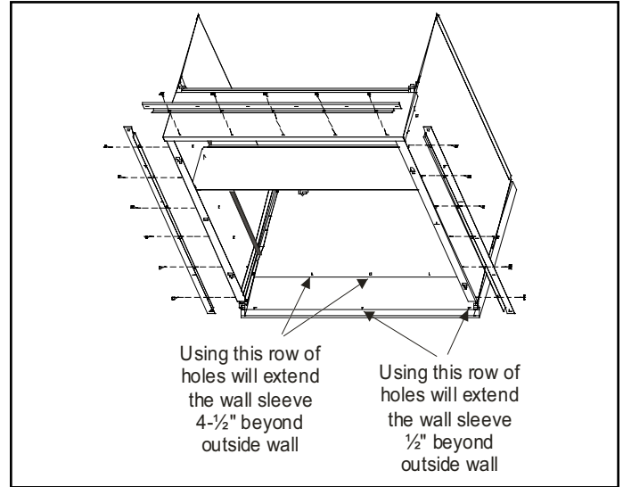
Figure 7. Installing Mounting Angles
