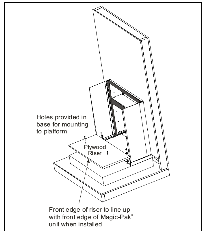
Figure 11. Attaching Base and Riser to Platform
