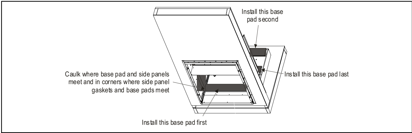
Figure 14. Installing Base Pads
