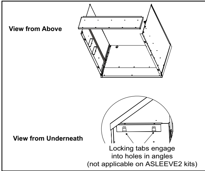
Figure 4. Attaching Top Panel
