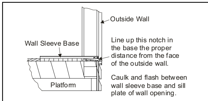
Figure 9. Positioning Wall Sleeve
